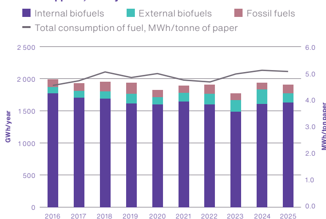
Fuel supplied, GWh/year
